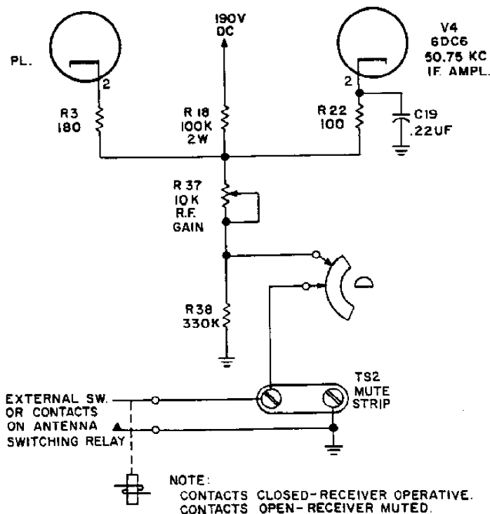
Figure 5. Schematic Diagram of Remote Receive-Standby Circuitry
